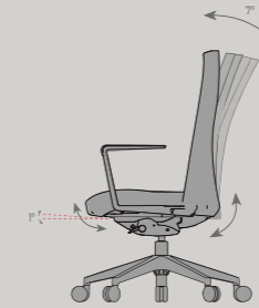
SYNCHRO MECHANISM TILT RATE Backrest tilt rate 7° to seat tilt rate 1° Auto-weight synchro control
