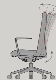
BACK TILT 4 back tilt positions. Tilt angles from 10° at the up-right blocked position up to 30° at the maximum angle
