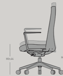
SEAT HEIGHT ADJUSTMENT. GAS LIFT Lowest seat height: 44 cm Maximum seat height: 54 cm
